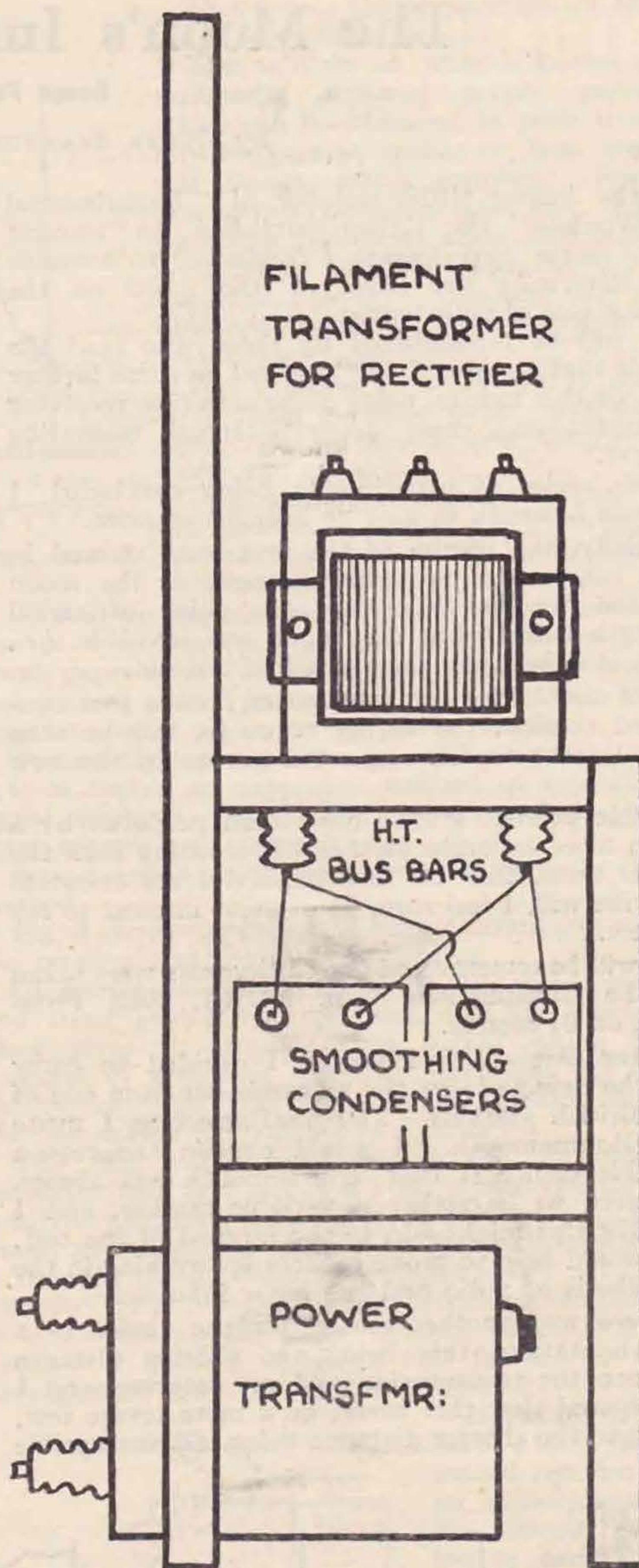
SIDE VIEW OF RECTIFIER PANEL
